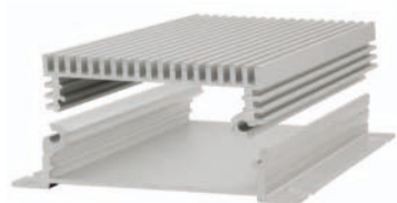
Filotec enclosures with cooling fins on one half-shell and moulded-on wall brackets on the other half-shell
